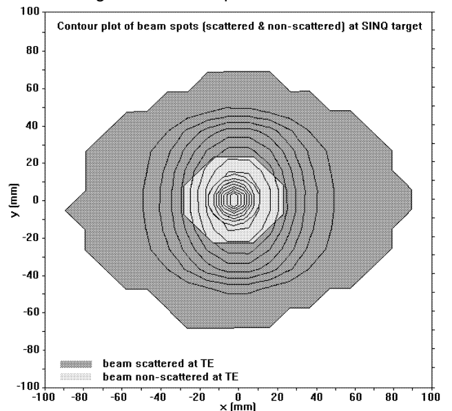
Fig. 9: Scattered an non-scattered beam-spot at SING
