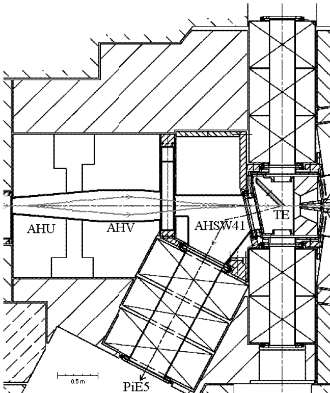
Fig. 10: AHU/AHV/AHSW41-magnets layout at TE
