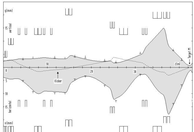
Fig. 4: The 2\sigma beam envelope of the newly adapted optics for the proton beam between the extraction of the 590 MeV Ring Cyclotron and Target M. The 2\sigma half-width in x at the location of the kicker is around 10 mm. The measured 2\sigma beam profile half-widths are indicated as T-symbols. The fit of the beam envelope to these data was done with the program Transport [7]. All drawn magnet aperture dimensions are scaled by a factor of 0.25. The dotted line represents the 0.1 % dispersion trajectory.
